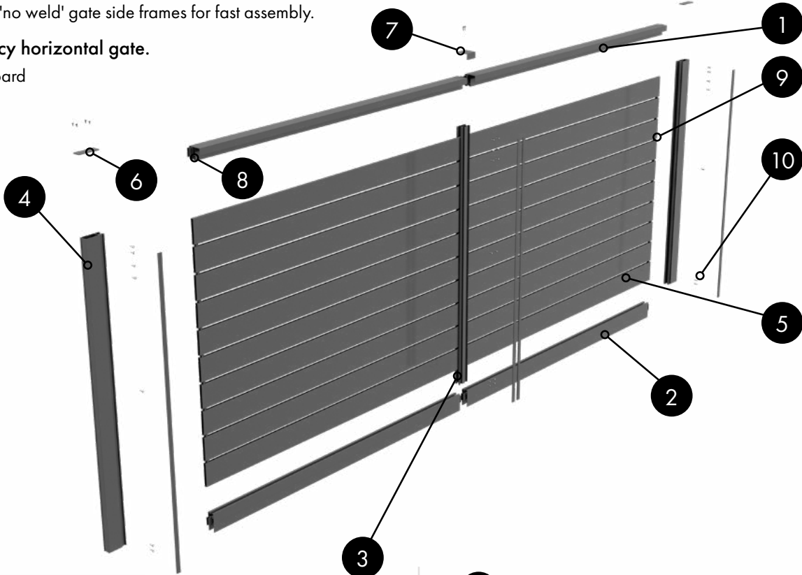
2 Sliding gate bottom rail 71" or 95" long Order Code: QSSG-1828/2413-BR
