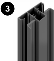
3 Heavy Duty Mid Rail Order Code: QSSG-MIDRAIL-2248 Used to join multiple panels together to create sliding gate - also used in horizontal application to create multiple designs
